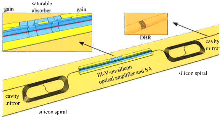
Fig. 17. Illustration of the linear cavity colliding pulse mode-locked laser.
