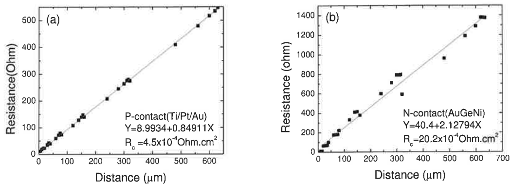
Figure 9: Resistance measured as a function of the distance between contact pads (a) P-contact (b) N-contact
