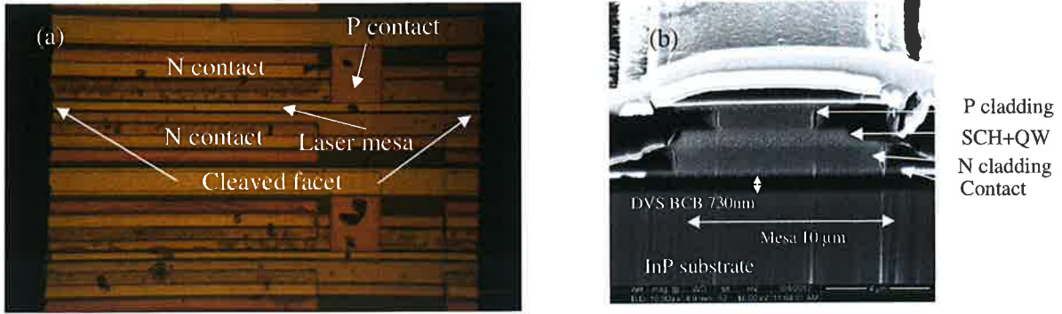
Figure 4: (a) optical image of the cleaved laser bar (b) SEM image of one of the laser cross sections
