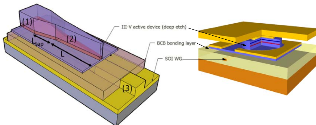
Figure 2: Heterogeneously integrated lasers. Left: transition section of a stripe laser. Right: Microdisk laser.
