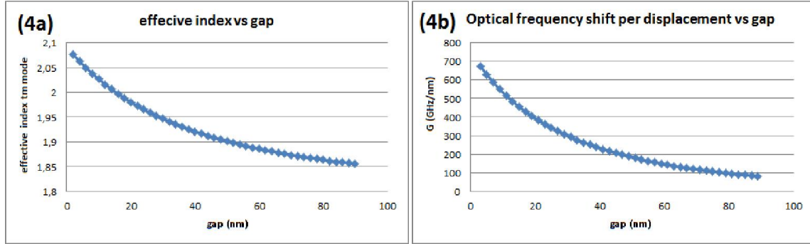
Figure 4: a) Finite element simulation of the effective index of the TM mode for different gap. b) Frequency shift per displacement G for different gaps.
