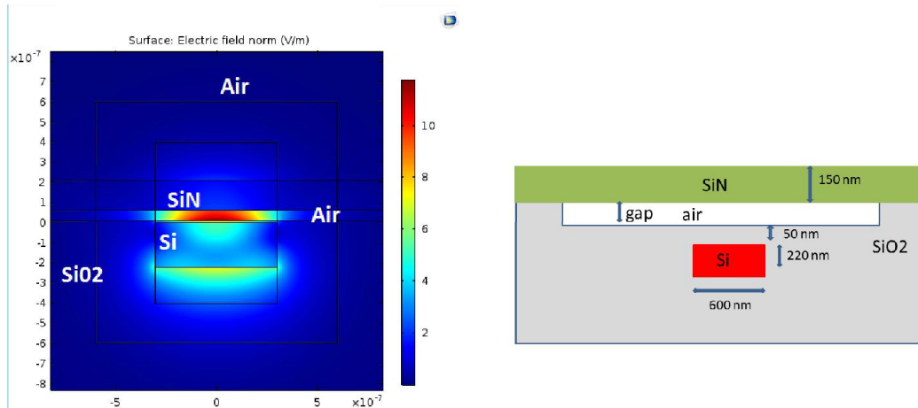
Figure 2: Optical mode (left) and cross-section of the resonator (right).
