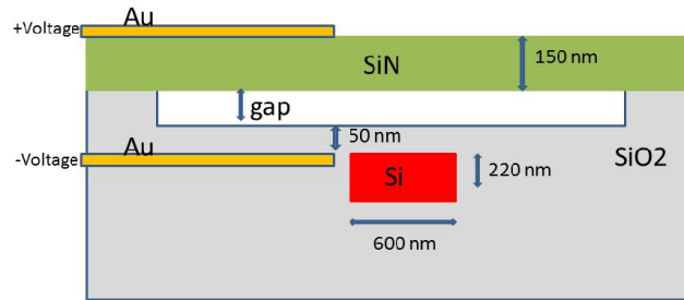
Figure 5: Cross section of the electrostatic tuning scheme.
