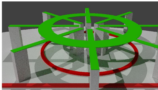
Figure 1: 3D view of the proposed design: in red the Si resonator and its bus waveguide, in green the SiN mechanical resonator.
