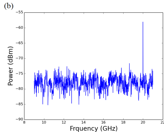
Fig. 2. Measured electrical spectra for (a) 8GHz to 16 GHz conversion and (b) 10 GHz to 20 GHz conversion.
