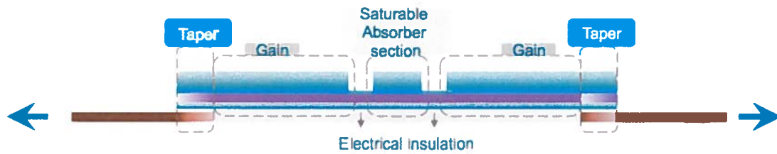
Fig. 2. Longitudinal cross-section of the III-V on silicon SOA/SA section
