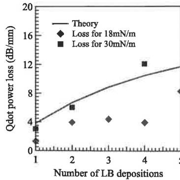
Figure 3: PbS/CdS Qdot losses at 1.55μm showing good agreement with simulations for a deposition at 30mN/m confirming the creation of a close packed layer on PWGs.
