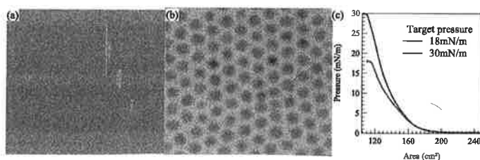
Figure 1: (a) Top view of the oxide planarized SOI waveguides.(b) TEM picture of PbS/CdS Qdots. (c) LB-isotherms for target pressures of 18 and 30mN/m.
