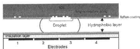
Figure 3: Incorporation of the SOI chip containing an array of microring resonator sensors into the digital microfluidic system by replacing the top glass plate of the platform.
