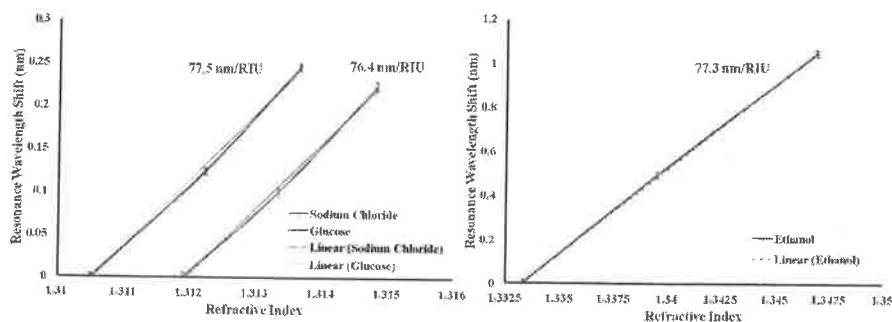
Figure 4. Three experiments with different sodium chloride, glucose and ethanol concentrations were performed. Each line corresponds to one of these experiments. Error bars indicate the standard deviations based on 3 repetitions. The sensitivity is determined to be 77\pm 0.6 nm/RIU [4].
