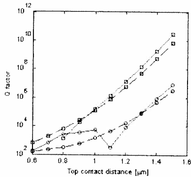
Figure 3: Q factor versus the top contact distance. Au is blue solid line, Ti is black dashed line. Square markers for the fundamental mode and round markers for the first order mode.
