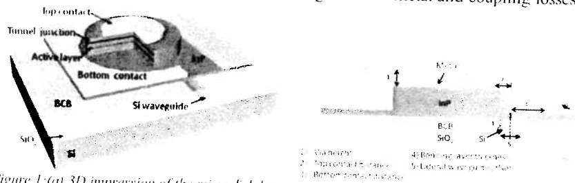
Figure 1: (a) 3D impression of the microdisk laser structure. (b) Cross-section of the microdisk laser with the relevant design parameters.
