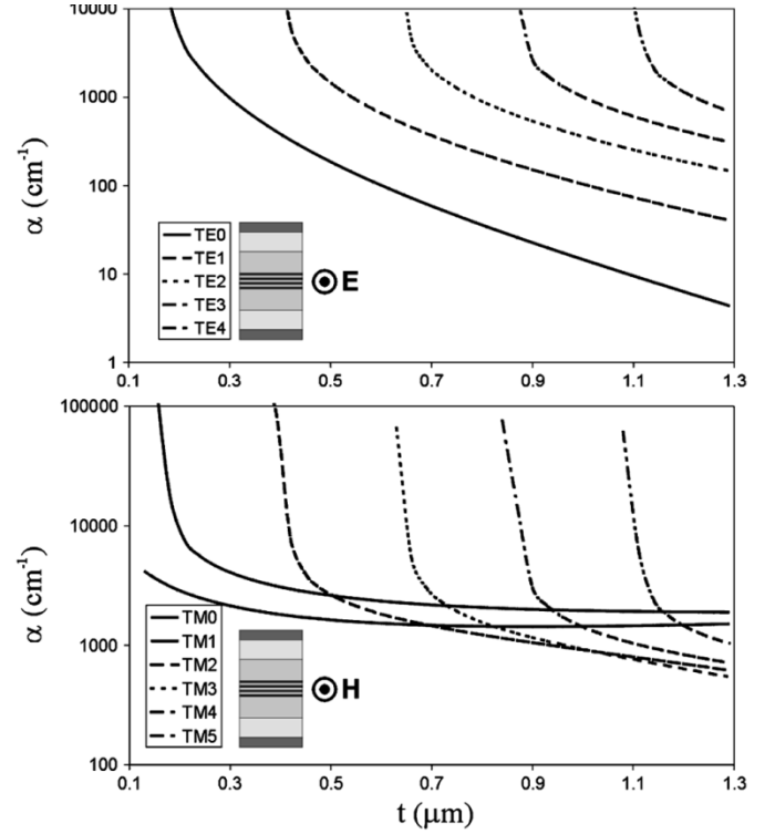
Fig. 2. Modal absorption losses of the fundamental and higher order modes of the waveguide structure as depicted in Fig. 1 (without patterning), at 1.5 \mu\text{m} . The TM 0 and TM 1 modes are plasmon-like.
